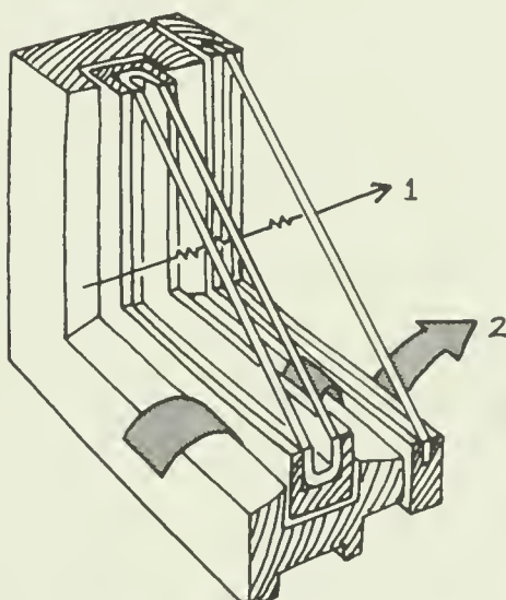
INSULATING GLASS WITH STORM WINDOW
