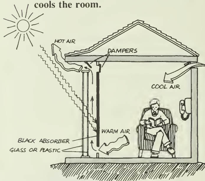
Chimney effect induces natural ventilation in summer.
