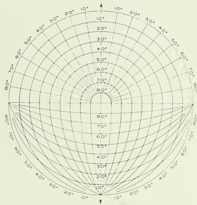
SHADING MASK PROTRACTOR
