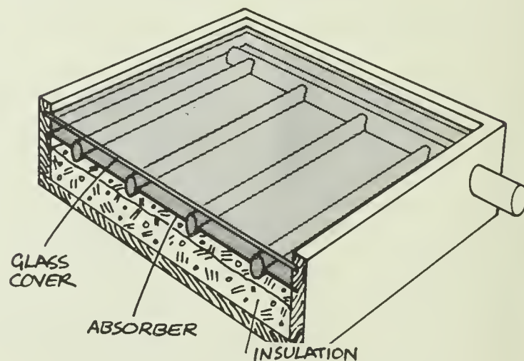
A liquid flat-plate collector.
