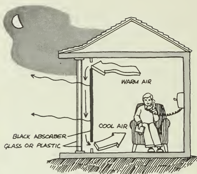
Undesirable reverse thermosiphoning cools the room.
