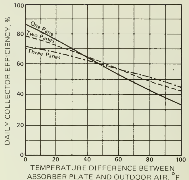
Performance of a moderately-insulated collector.
