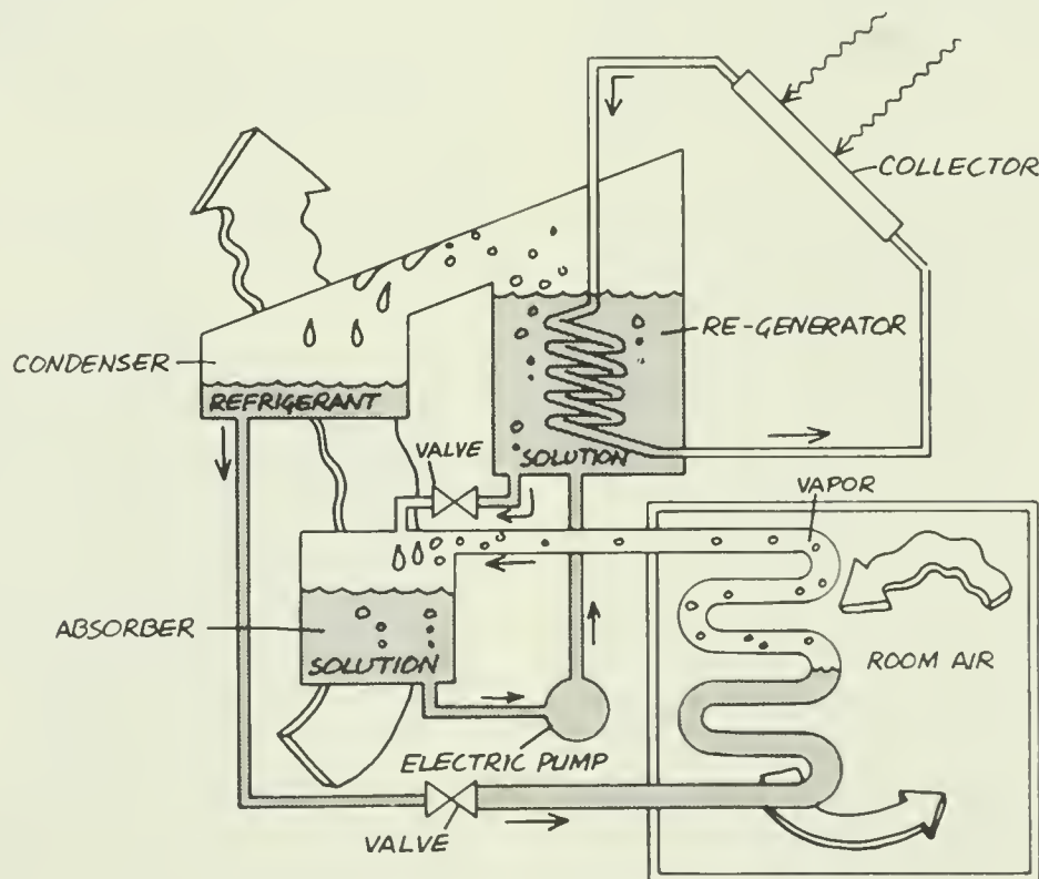
Absorption Cooling Cycle.
