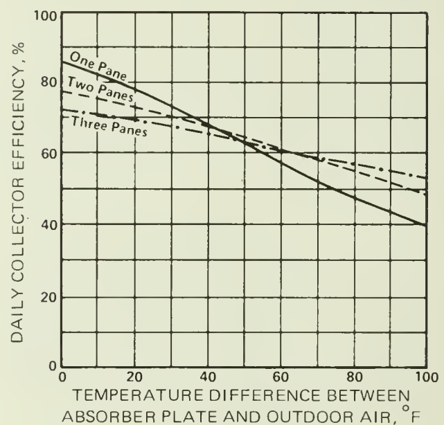
Performance of a well-insulated collector.
