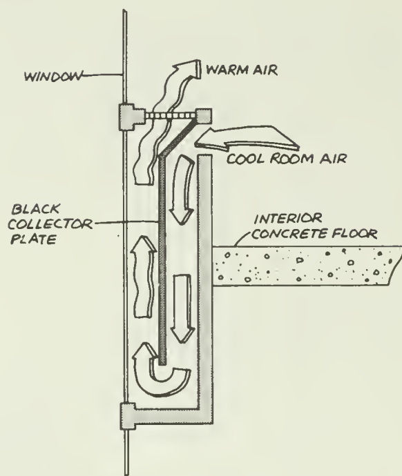
Cross-section of CNRS wall collector.
