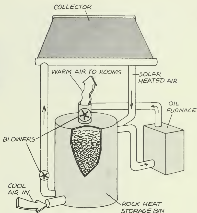
Schematic diagram of an air system with rock heat storage.
