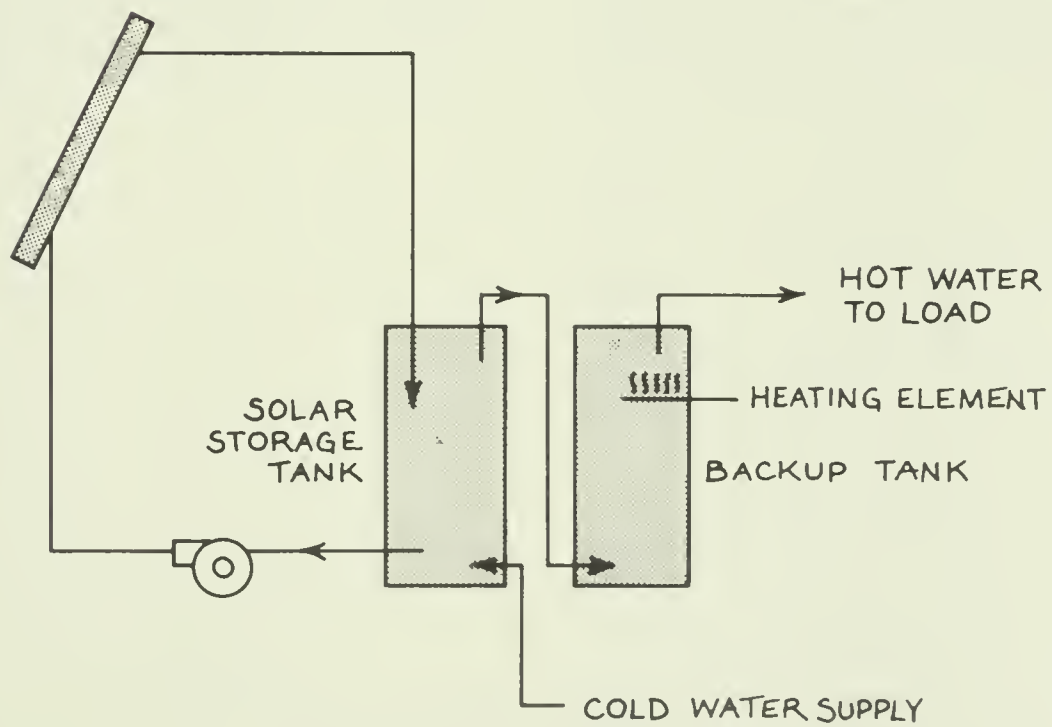
A two-tank solar DHW system.
