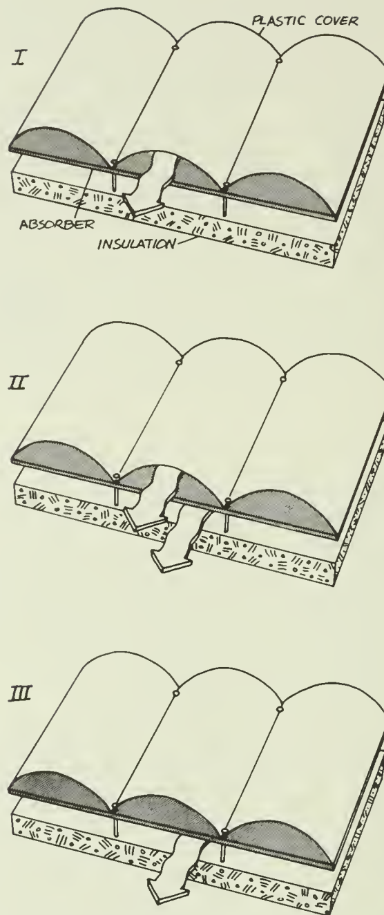
The three types of warm air solar collectors.
