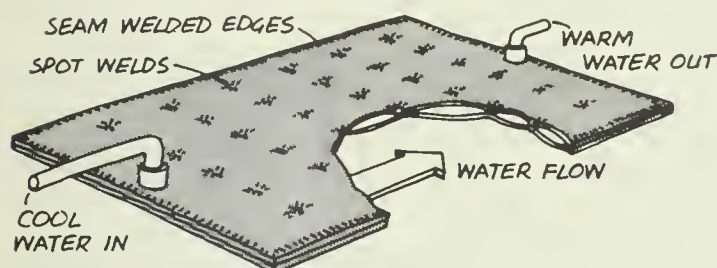
A typical sandwich-type absorber.
