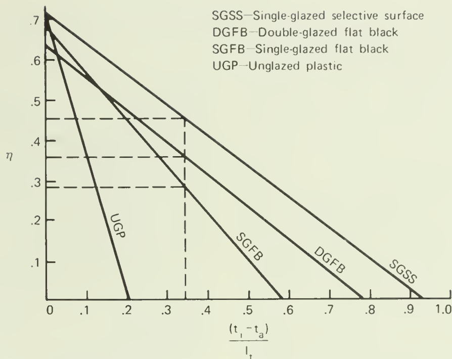
Four sample thermal efficiency curves. (Solar Age)
