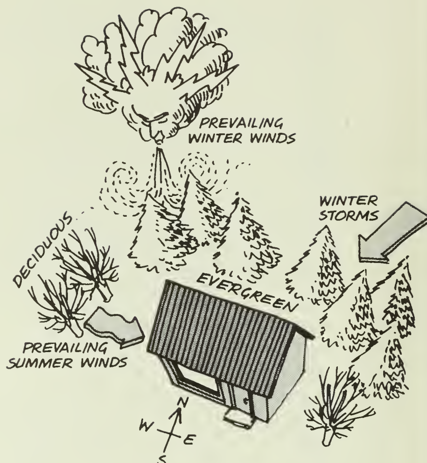
Proper orientation and vegetation shields protect a house from the wind.
