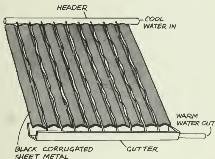
Thomason's trickle-down absorber.
