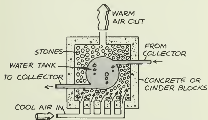
This approach uses both water and stone as storage media.
