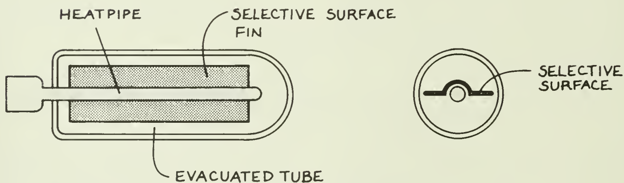
Heat pipe evacuated tube.
