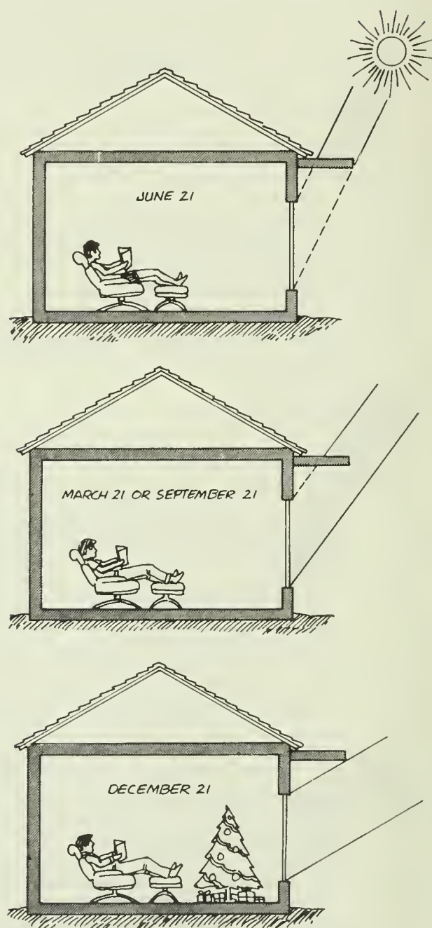
Shading a south window with a fixed overhang (at solar noon).
