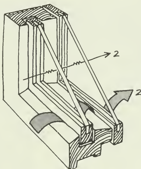
SINGLE GLASS WITH STORM WINDOW
