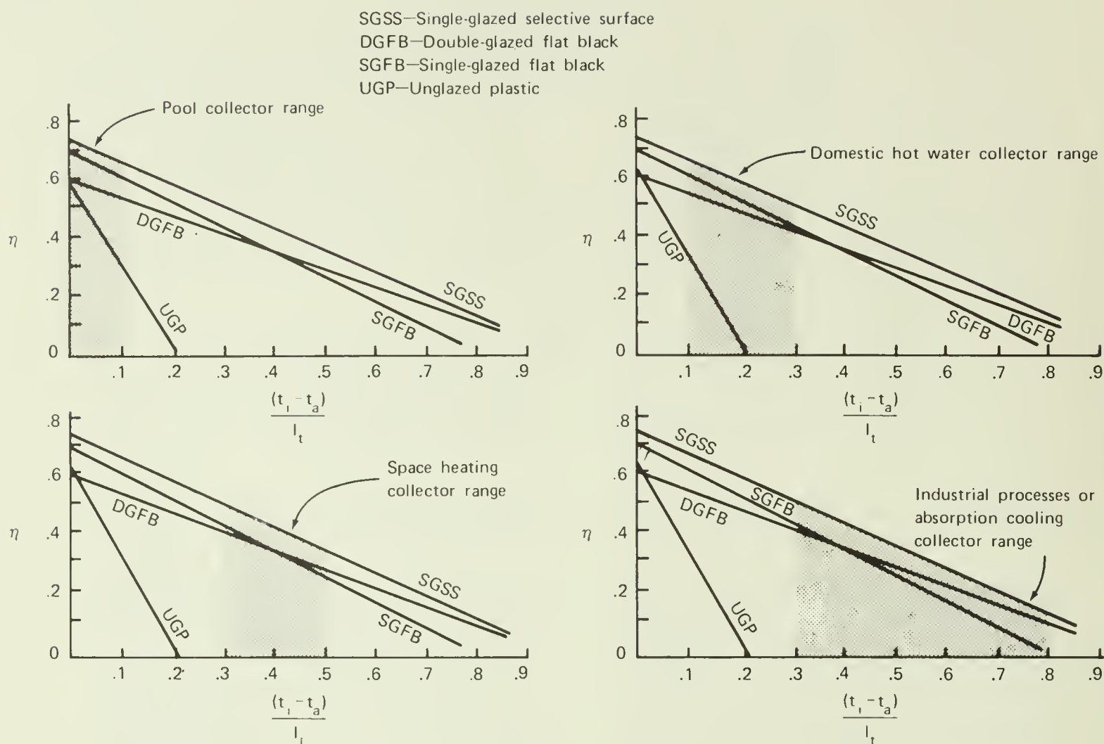
General fluid parameter boundaries for different applications. ( Solar Age )
