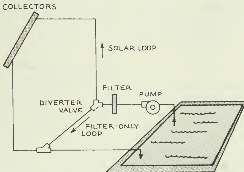
Solar swimming pool heating.
