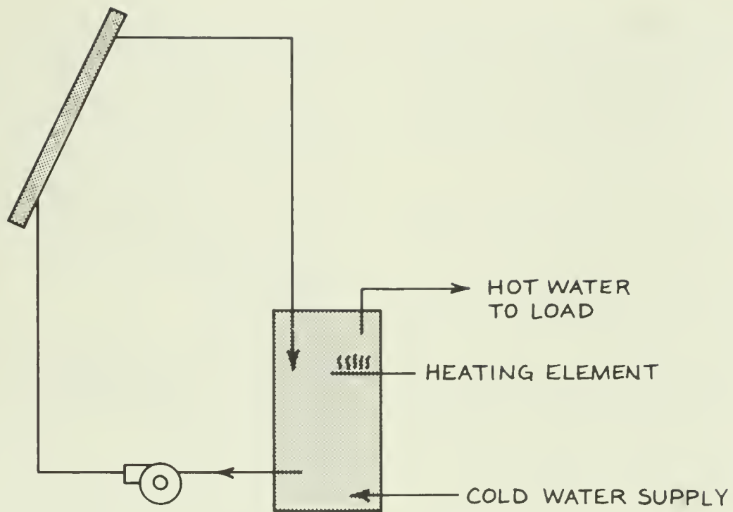
A one-tank solar DHW system.
