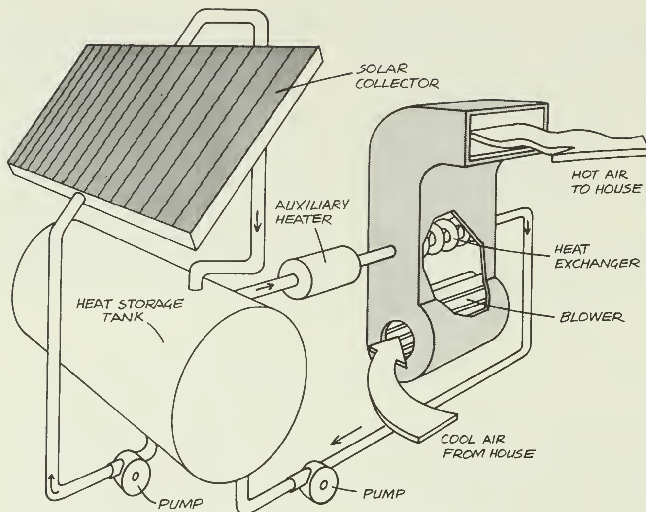
A typical active system for solar heating.
