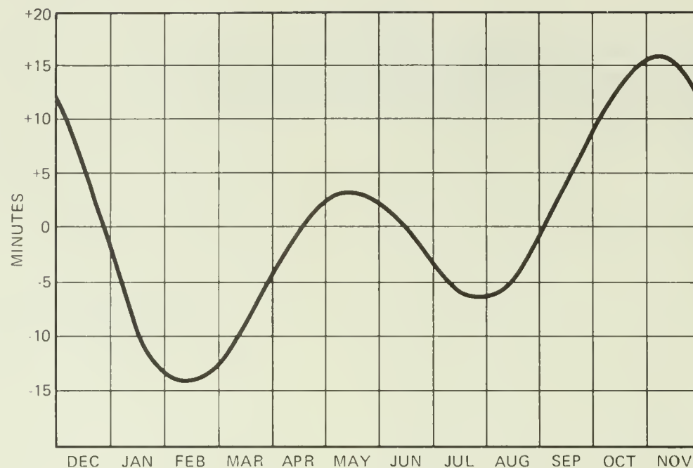
Equation of time
