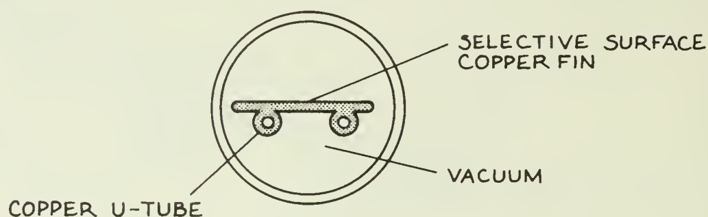
Subsequent evacuated tube design.
