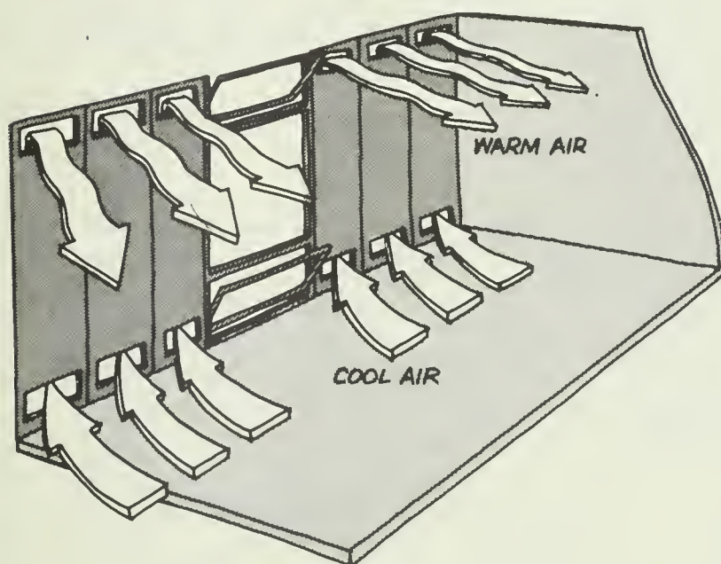
A thermosiphoning air collector—two views.
